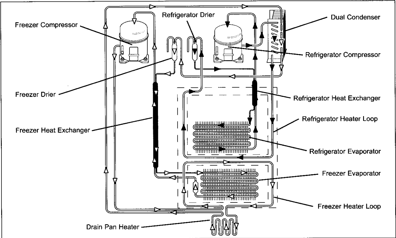
Figure 4-9. Models 611-3, 611G-3, 650-3, 650G-3 Refrigerant Flow
