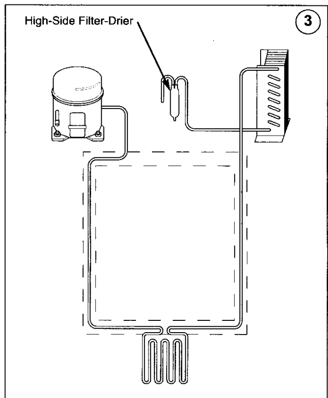
Figure 4-3. High-Side Filter-Drier
