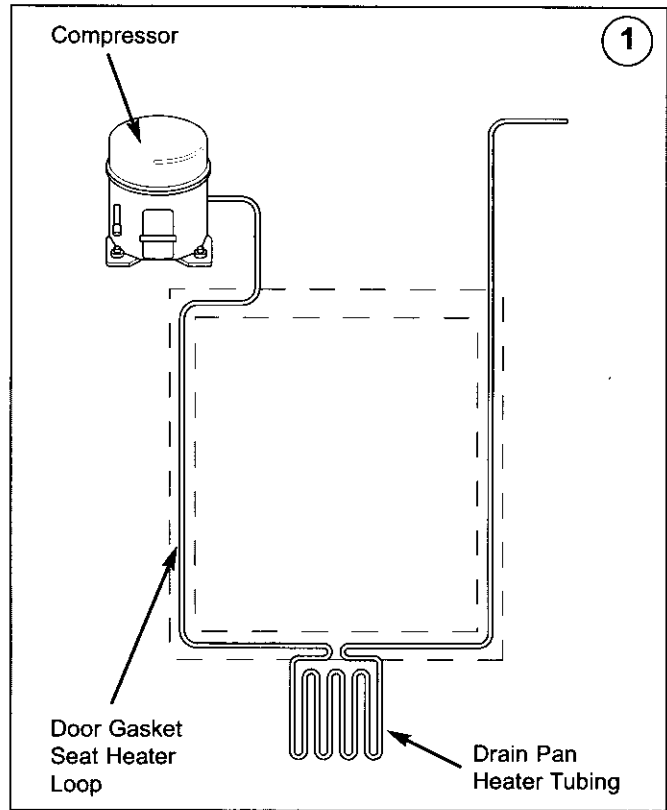
Figure 4-1. Compressor
