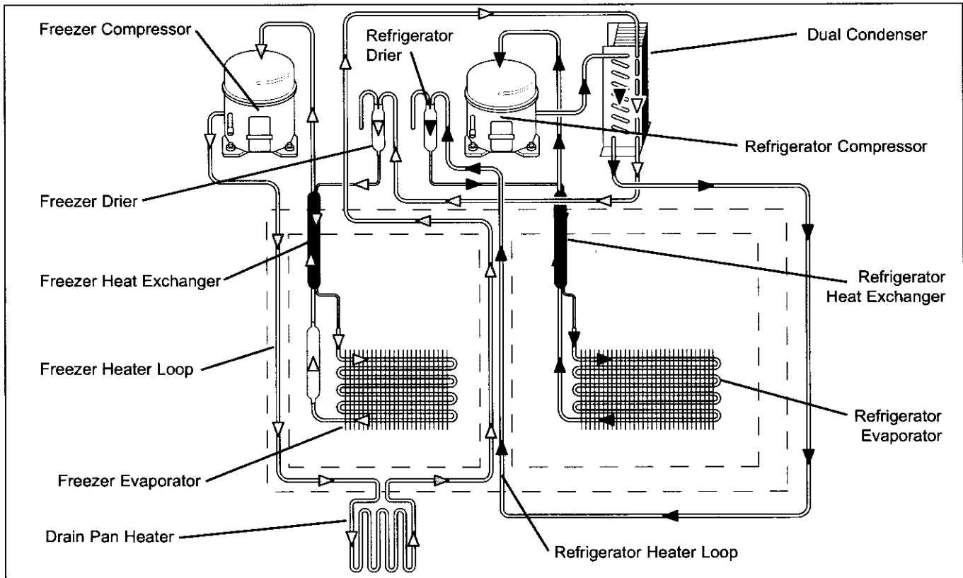
Figure 4-10. Models 632-3, 642-3, 661-3, 685-3, 695-3 Refrigerant Flow
