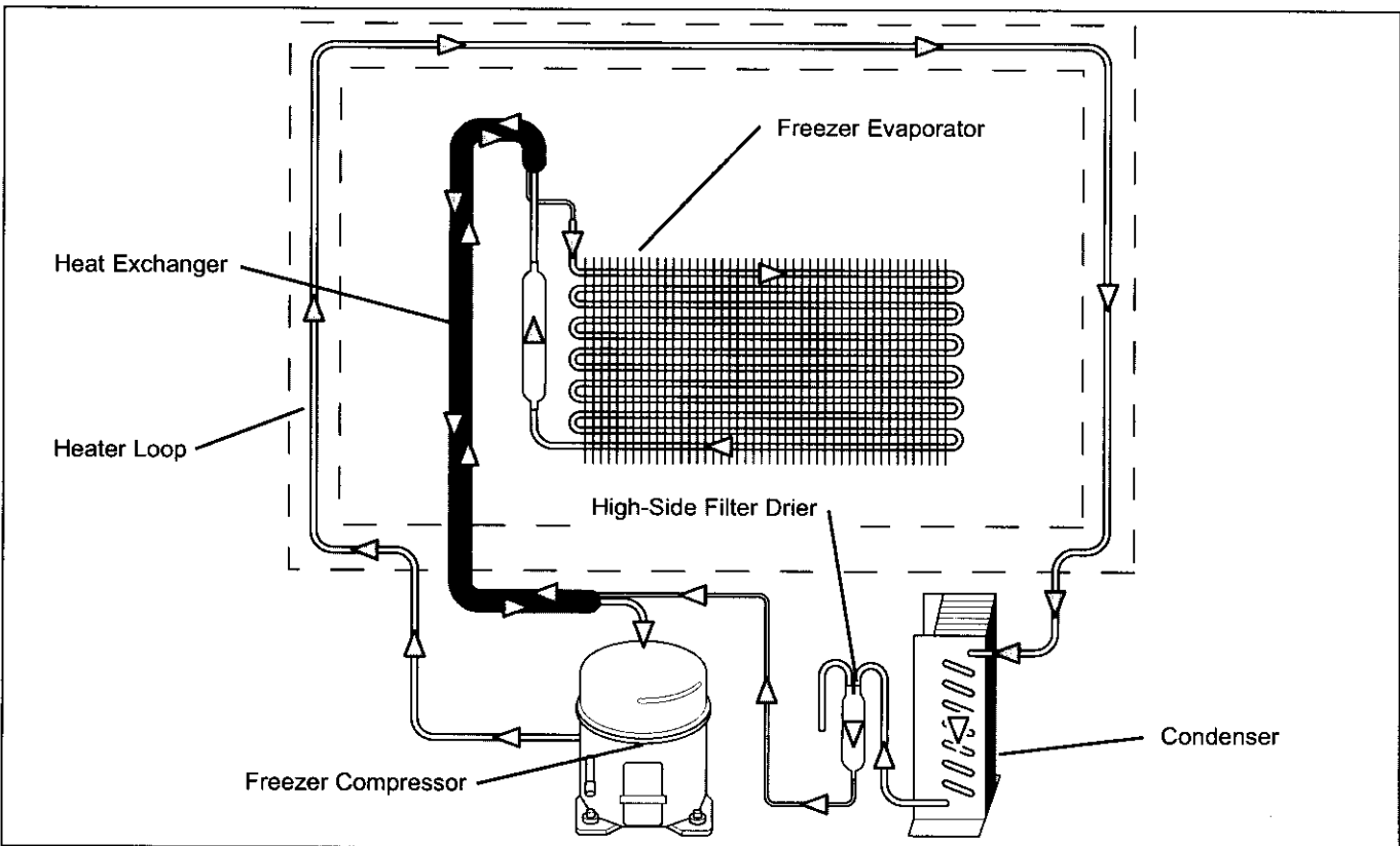
Figure 4-8. Model 601F-3 Refrigerant Flow
