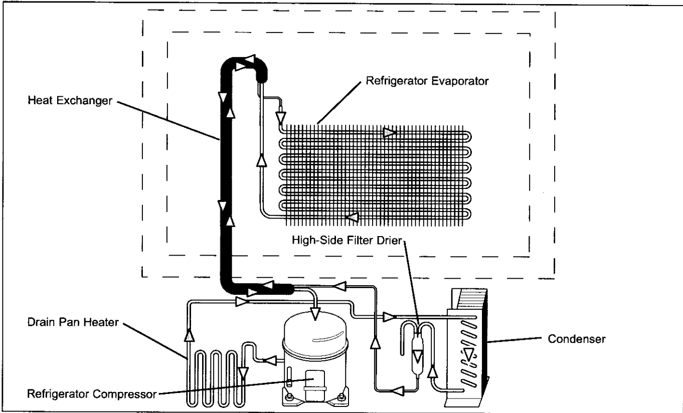
Figure 4-7. Models 601R-3, 601RG-3 Refrigerant Flow
