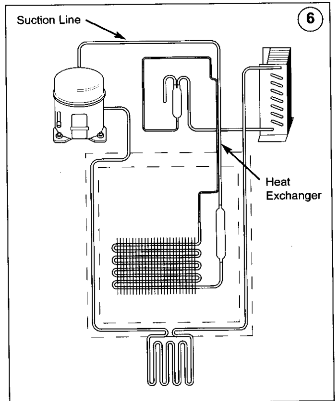
Figure 4-6. Suction Line (Part of Heat Exchanger)
