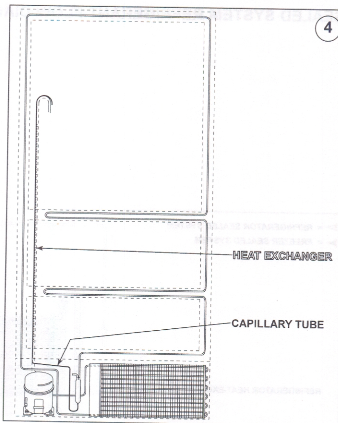
Figure 4-4. Capillary Tube (&amp; Heat Exchanger)
