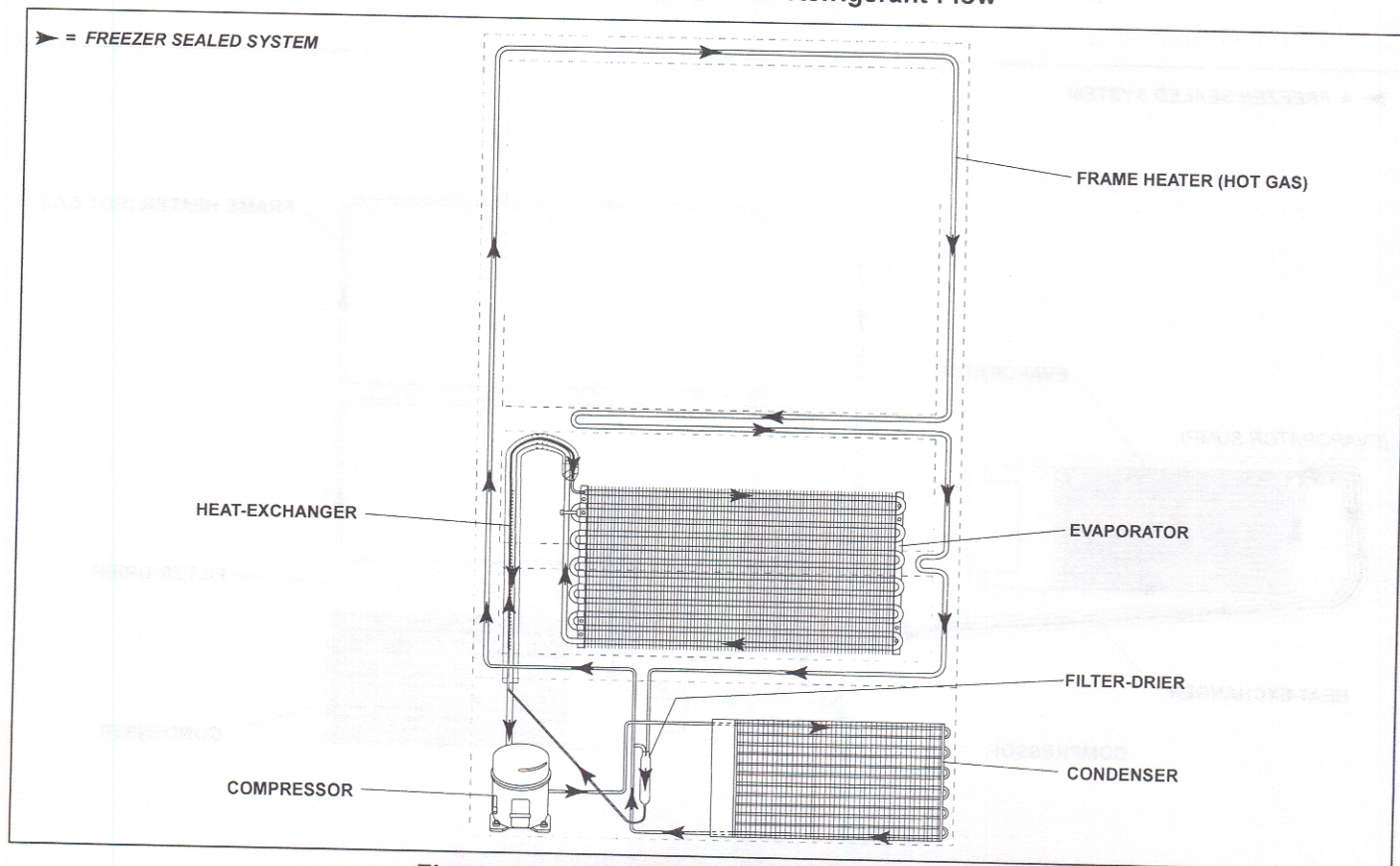
Figure 4-9. Model 700TF/I-2 Refrigerant Flow
