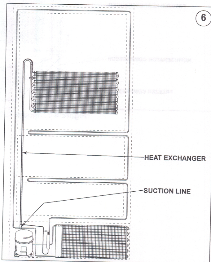
Figure 4-6. Suction Line &amp; Heat Exchanger
