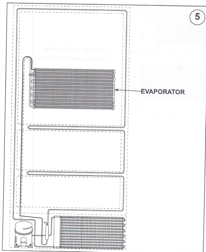
Figure 4-5. Evaporator
