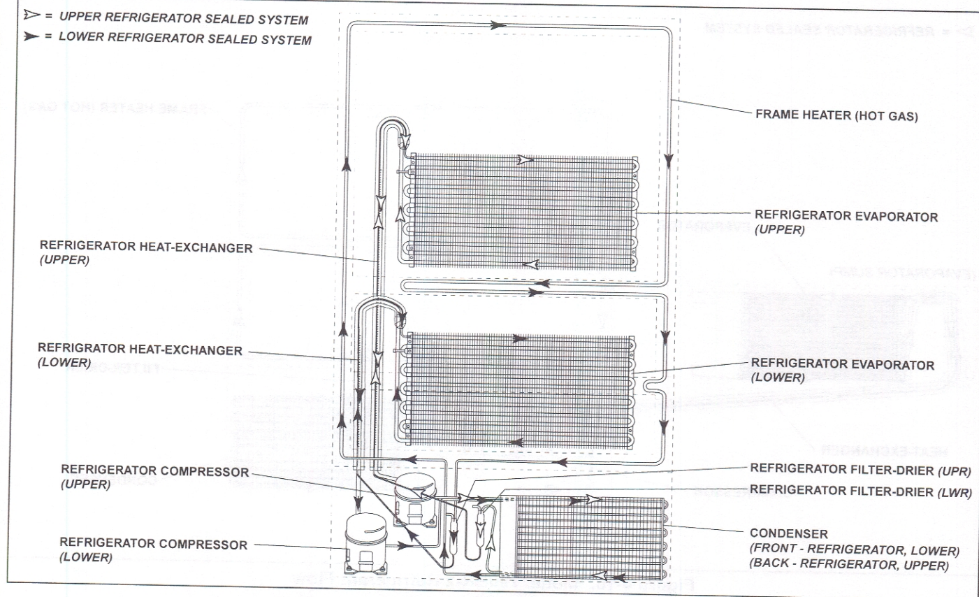
Figure 4-8. Model 700TR-2 Refrigerant Flow
