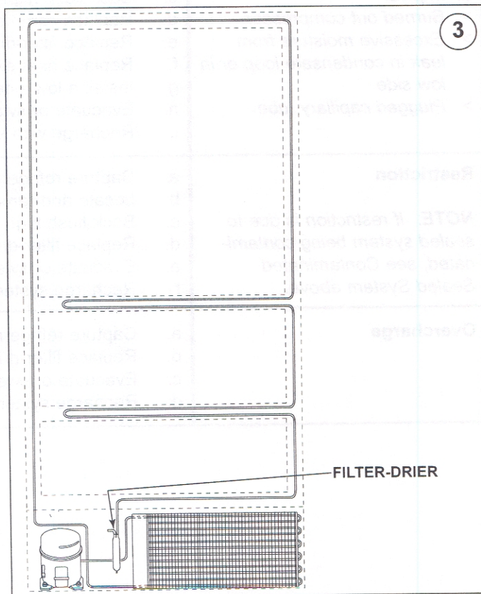
Figure 4-3. Filter-Drier
