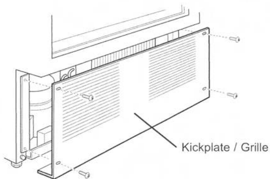
Figure 2-1. Kickplate/Grille Removal
