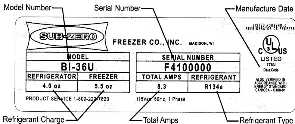
Figure 1-1. Serial Tag Layout (Layout Reference Only)
