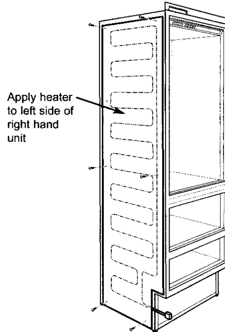
Figure 2-6. Dual Unit Heater (#TTDUAL Shown)
