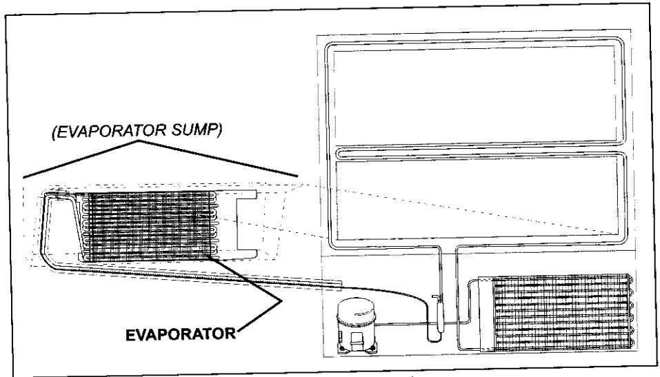
Figure 4-5. Evaporator
